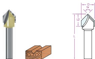
V-Nutfräser V-Groove Bit
